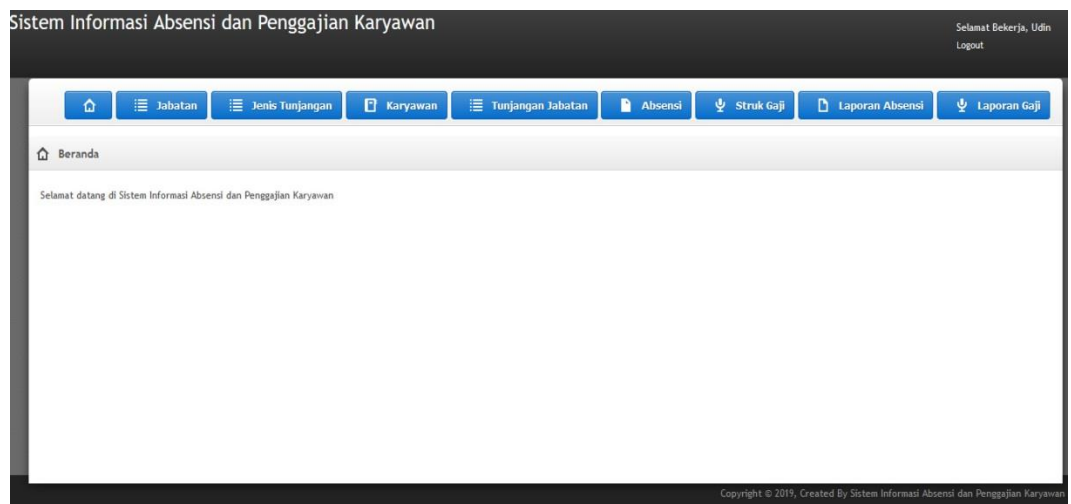
Gambar III.33 Halaman Home
