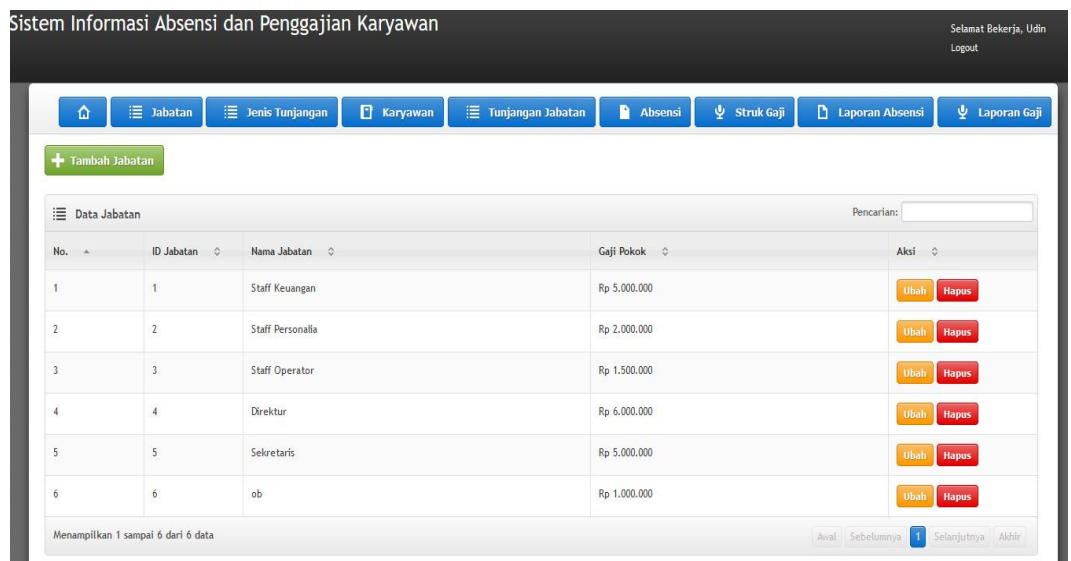
Gambar III.34 Halaman Jabatan
