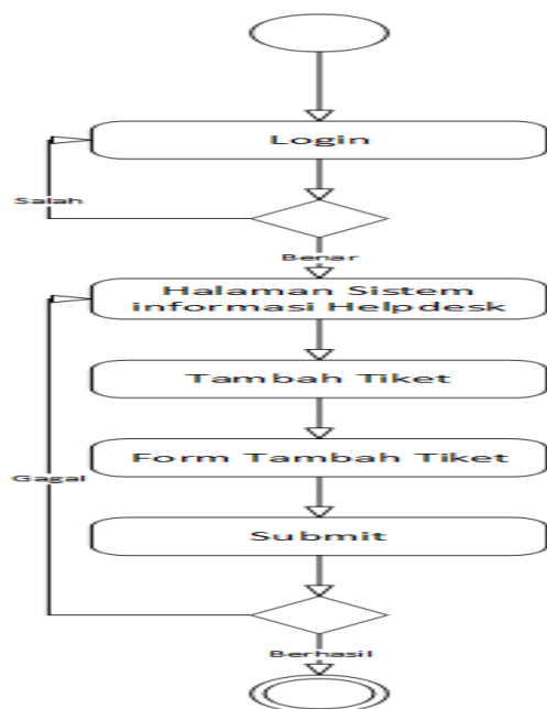
Figure 5 Activity Diagram Create New Ticket
