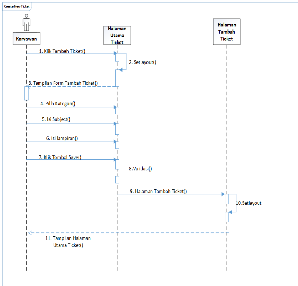
Figure 11 Sequence Diagram Create New Ticket
