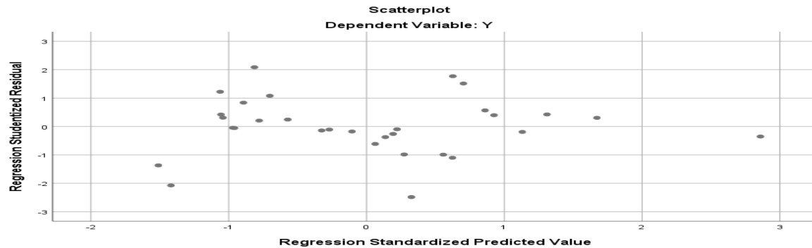
Figure 9: Heteroscedasticity Test Results
