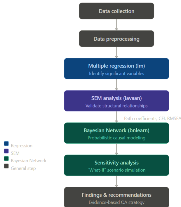
Figure 1. Flowchart Method
