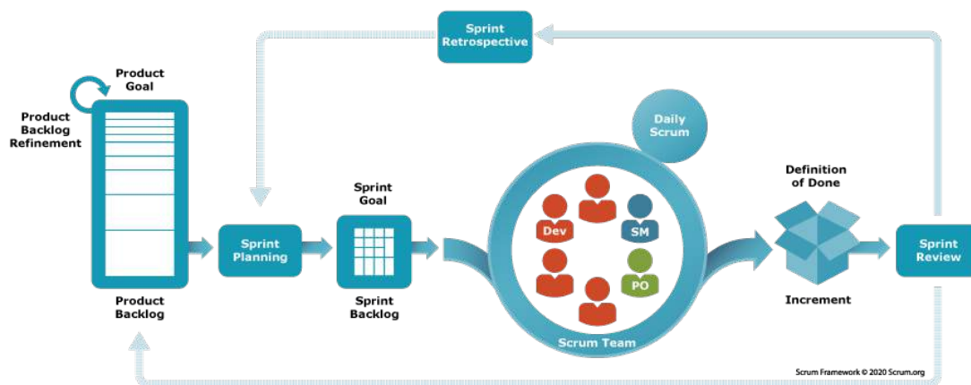
Gambar 1. Scrum Framework
