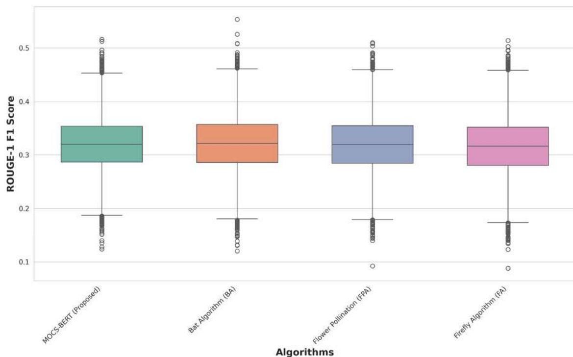
Figure 5. Distribution of ROUGE-1 Scores
