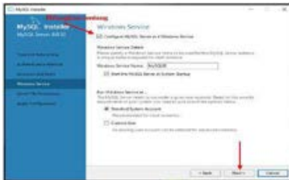
Gambar 7.12 Windows Service
