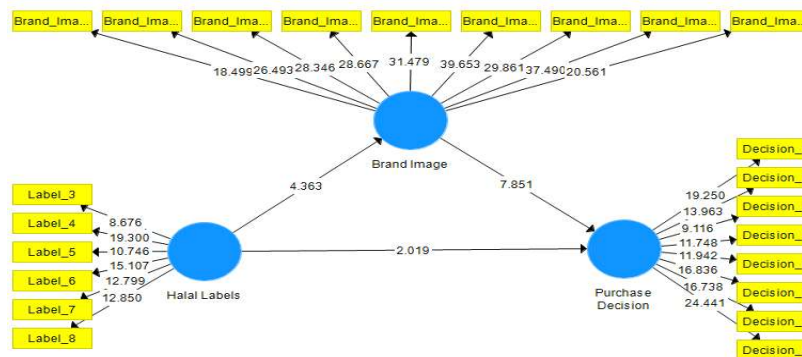
Figure 3. Bootstrapping
