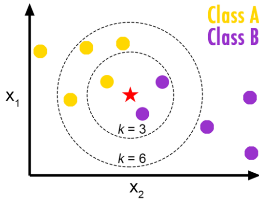
Gambar 6. Model KNN
