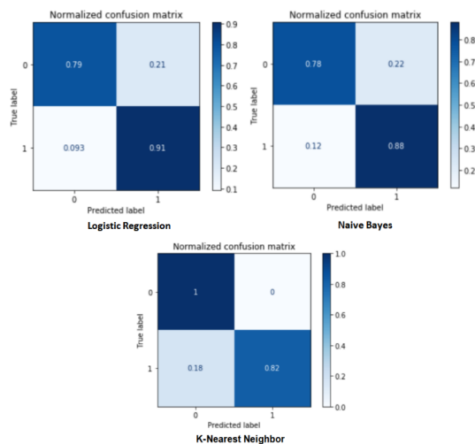
Gambar 11. Matrix Model Algoritma
