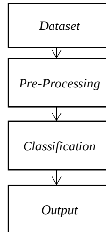
Gambar 1. Metode Penelitian
