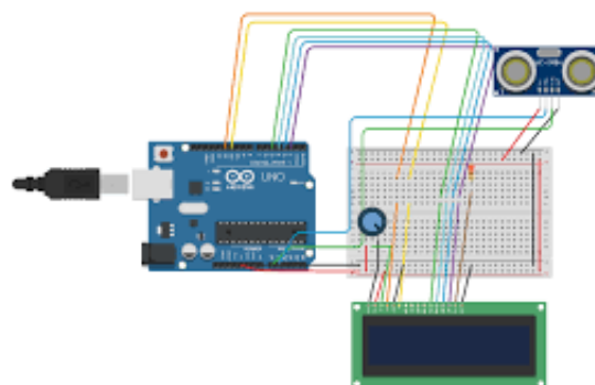
Gambar 1. Desain Wiring Prototype
