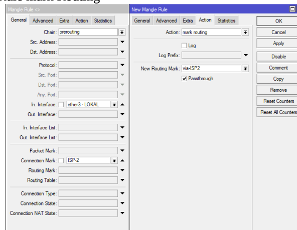
Gambar 7. Konfigurasi Rule mark Prerouting
