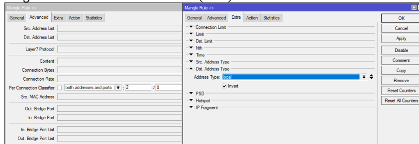
Gambar 6. Mangle Per Conneciton Classifier (PCC)
