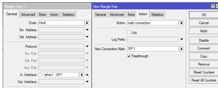
Sumber: Penelitian (2022) Gambar 3. Mangle Rule Input
