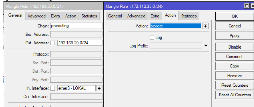
Gambar 5. Mangle rule output
