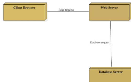
Gambar 4. Deployment Diagram
