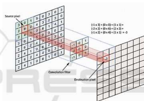
Figure 3: Visualization of convolution layer (Biswas and Islam, 2021).
