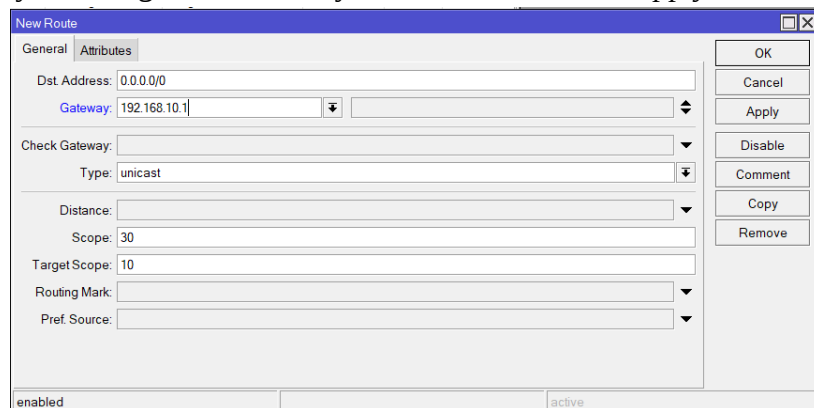
Gambar 15. Tampilan General
