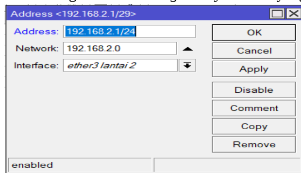
Gambar 14. Tampilan Address
