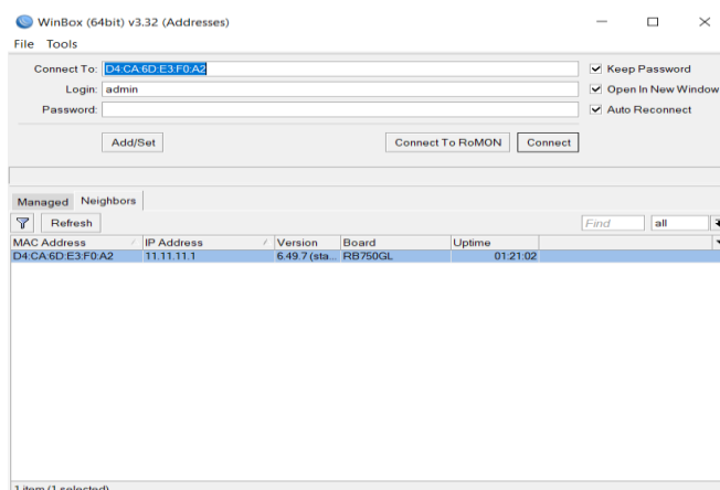
Gambar 9. Tampilan Winbox
