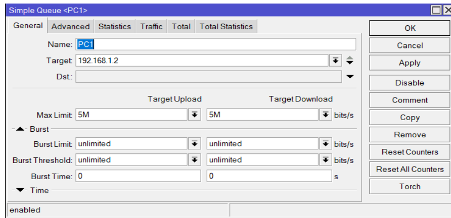
Gambar 18. Tampilan General
