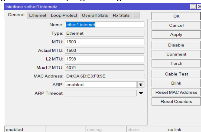
Gambar 10. Tampilan General
