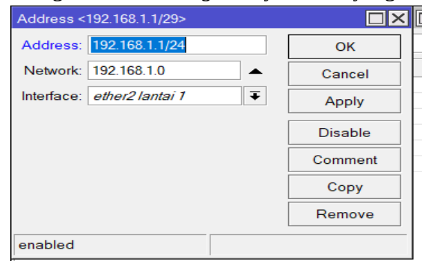
Gambar 13. Tampilan Address
