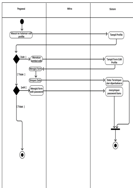
Gambar 3. Activity Diagram Menu Edit Profile
