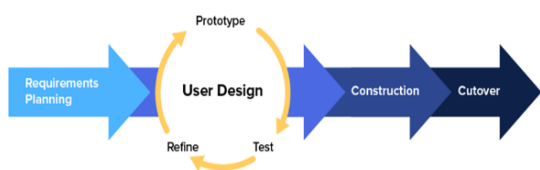
Gambar 1. Model Rapid Application Development (RAD)
