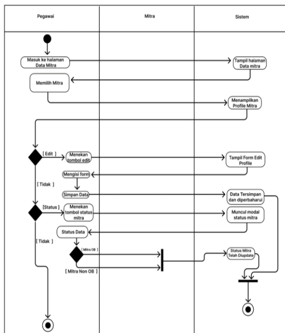
Gambar 4. Diagram Activity Menu Data Mitra.
