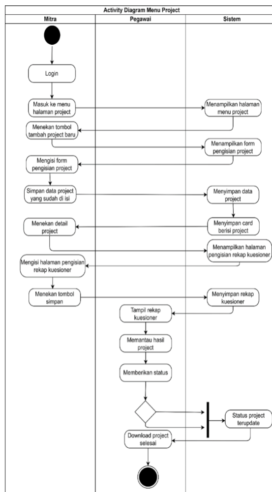
Gambar 5. Activity Diagram Menu Project Sumber : (Simpony et al., 2024)
