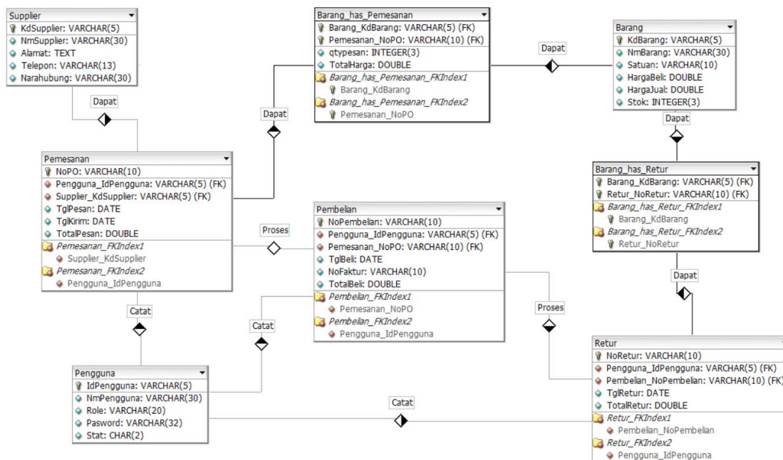
Gambar 4. Entity Relationship Diagram Sistem Pembelian Bahan Baku
