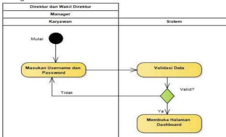
Gambar 5. Activity Diagram Login
