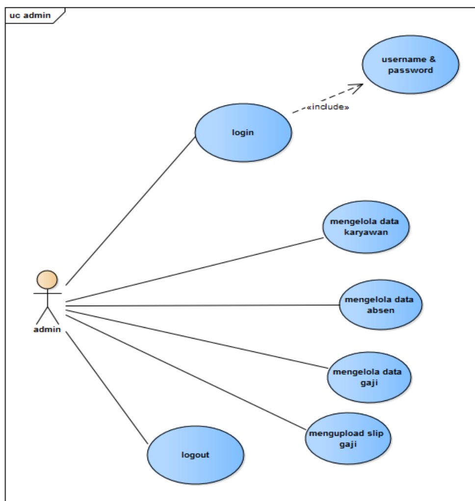
Gambar IV.2 Usecase Diagram Admin
