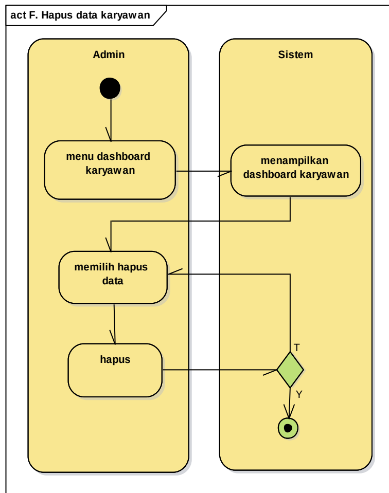
Gambar IV.8 Diagram Activity Hapus Data Karyawan
