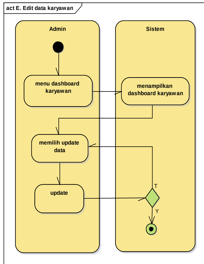
Gambar IV.7 Diagram Activity Update Data Karyawan
