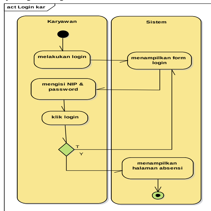
Gambar IV.3 Activity Diagram Login
