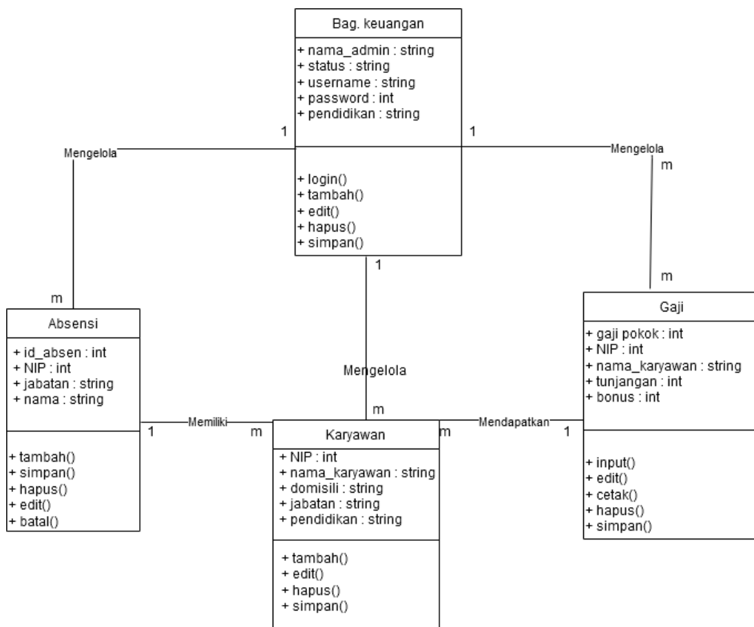
. Gambar IV.37. Class Diagram Sistem Usulan
