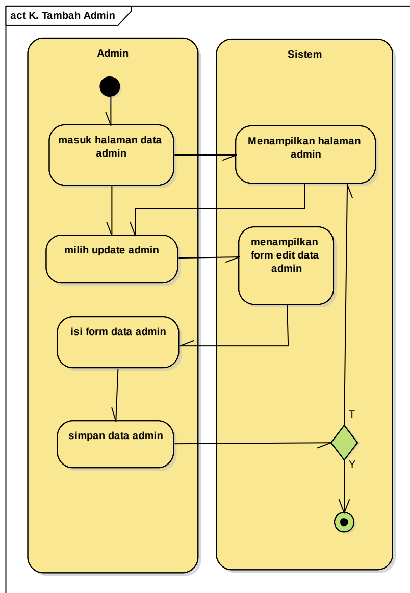
Gambar IV.13 Diagram Activity Tambah Admin
