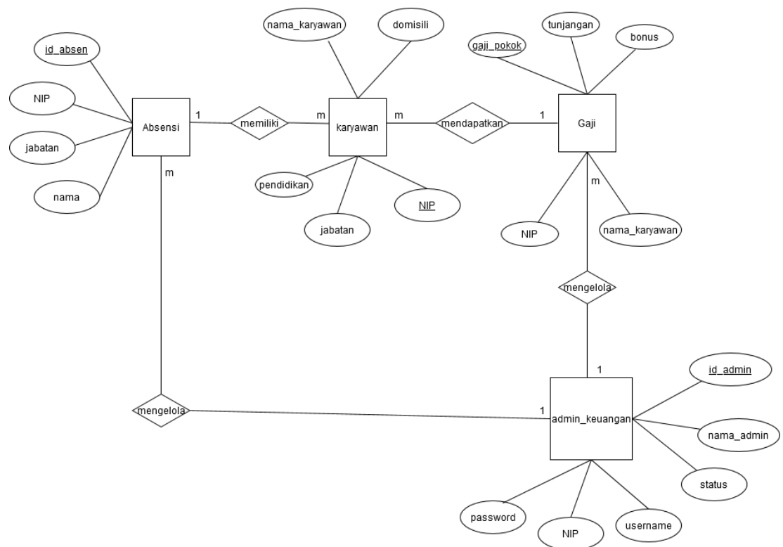
Gambar IV.35. Entity Relationship Diagram Sistem Usulan
