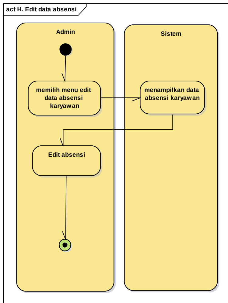
Gambar IV.10 Diagram Activity Edit Data Absensi Karyawan
