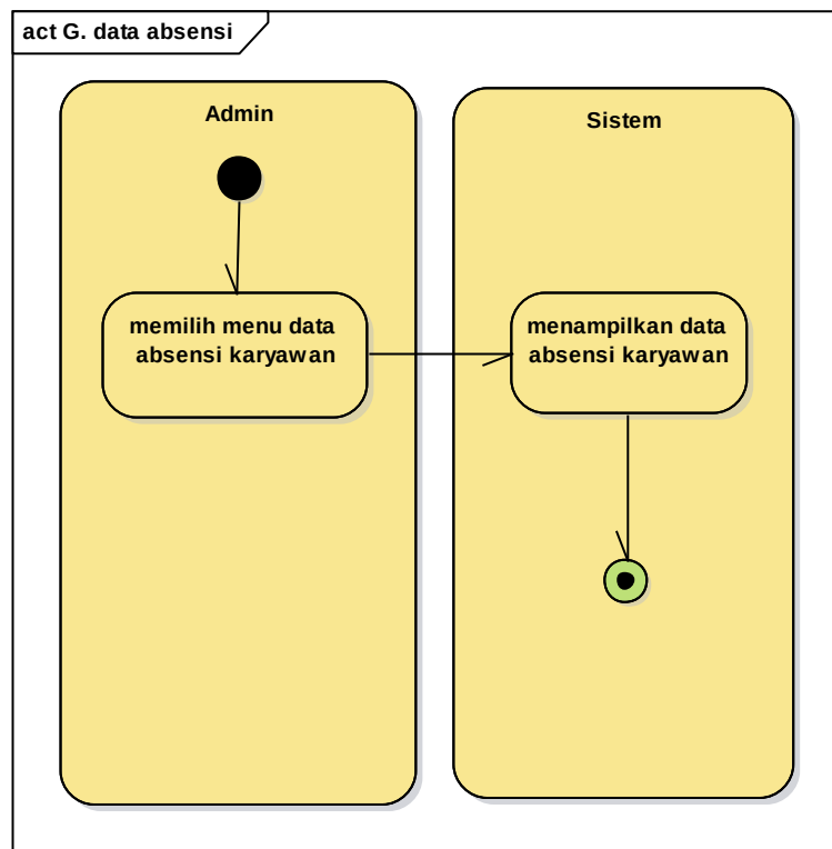
Gambar IV.9 Diagram Activity Data Absensi Karyawan
