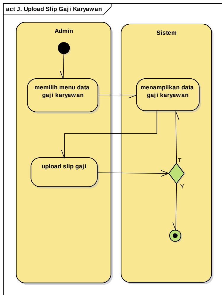
Gambar IV.12 Diagram Activity Upload Slip Gaji Karyawan
