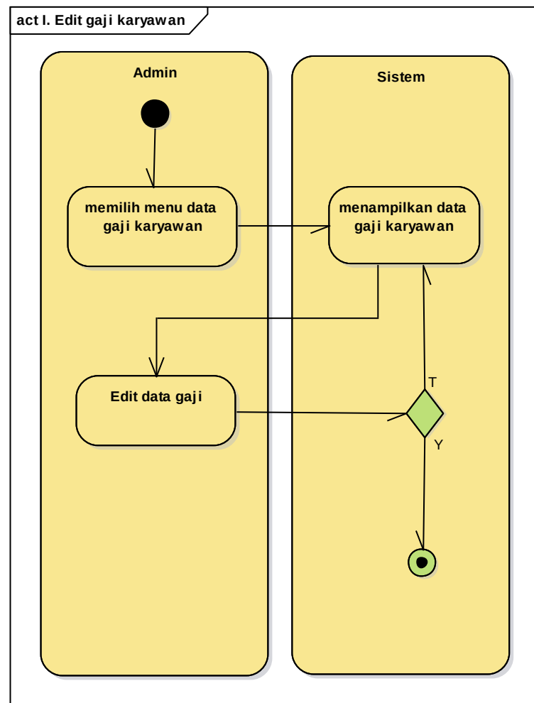
Gambar IV.11 Diagram Activity Edit Data Gaji Karyawan
