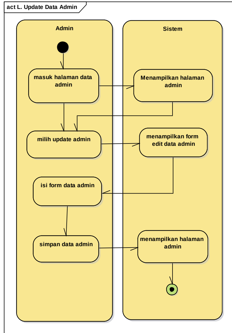
Gambar IV.14 Diagram Activity Update Data Admin
