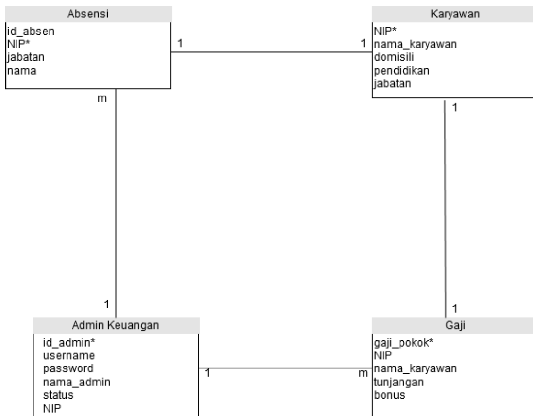
Gambar IV.36. Logical Record Structure (LRS) Sistem Usulan
