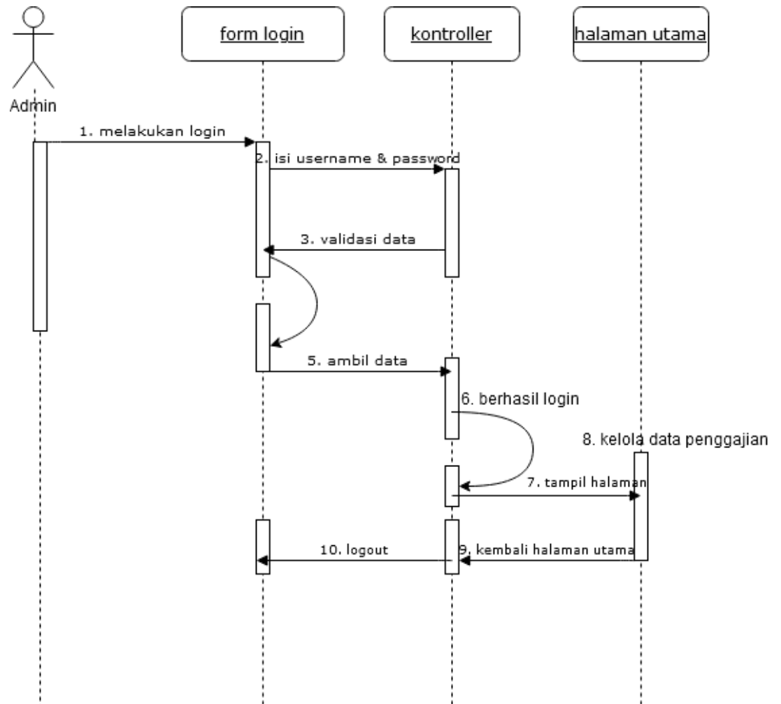
Gambar IV.38. Sequence Diagram Sistem Usulan
