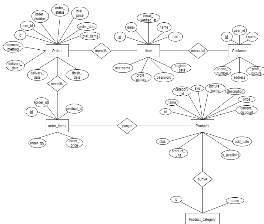
Gambar III.4 Entity Relationship Diagram (ERD)
