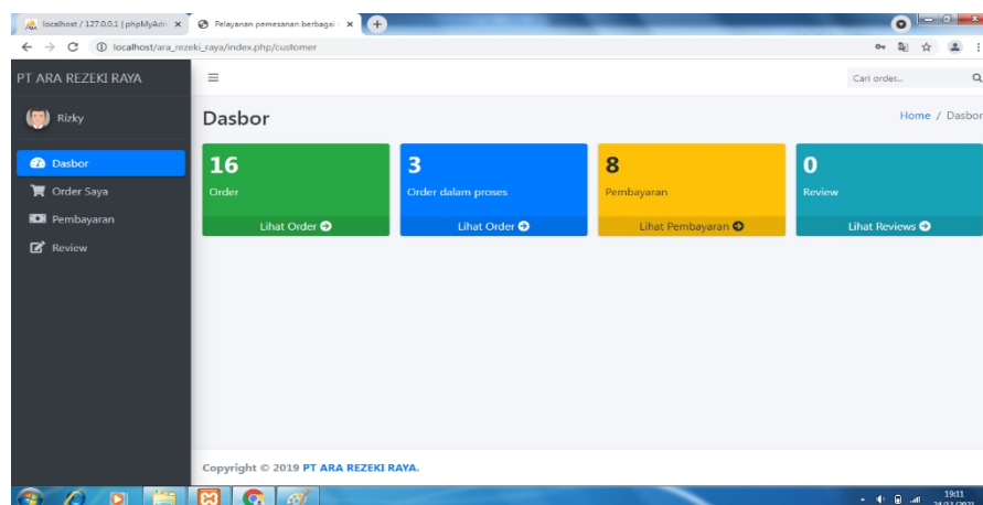
Gambar III.10.3 Halaman Costumer
