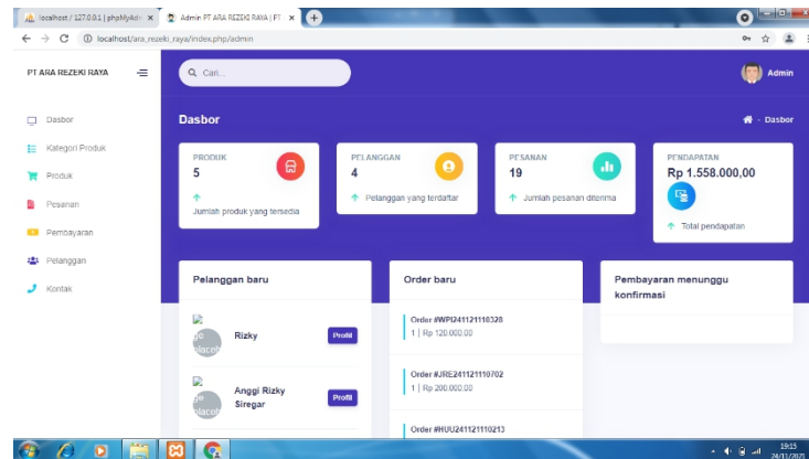
Gambar III.10.4 Halaman Admin
