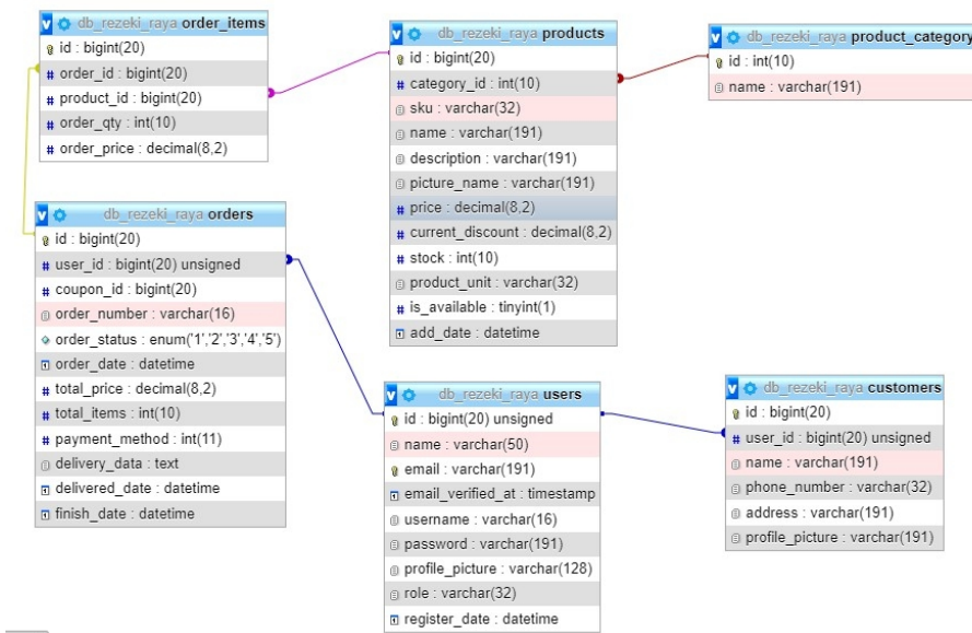
Gambar III.5 Logical Record Structure (LRS)
