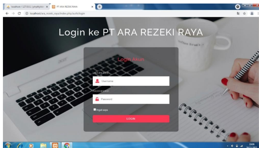
Gambar III.10.1 Halaman Login
