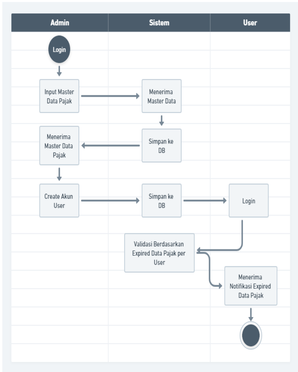
Gambar 4.1 Activity Diagram SI-MOJAKEMO
