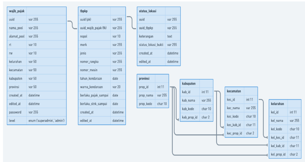
Gambar 4.10 Logical Record Structure (LRS) SI-MOJAKEMO
