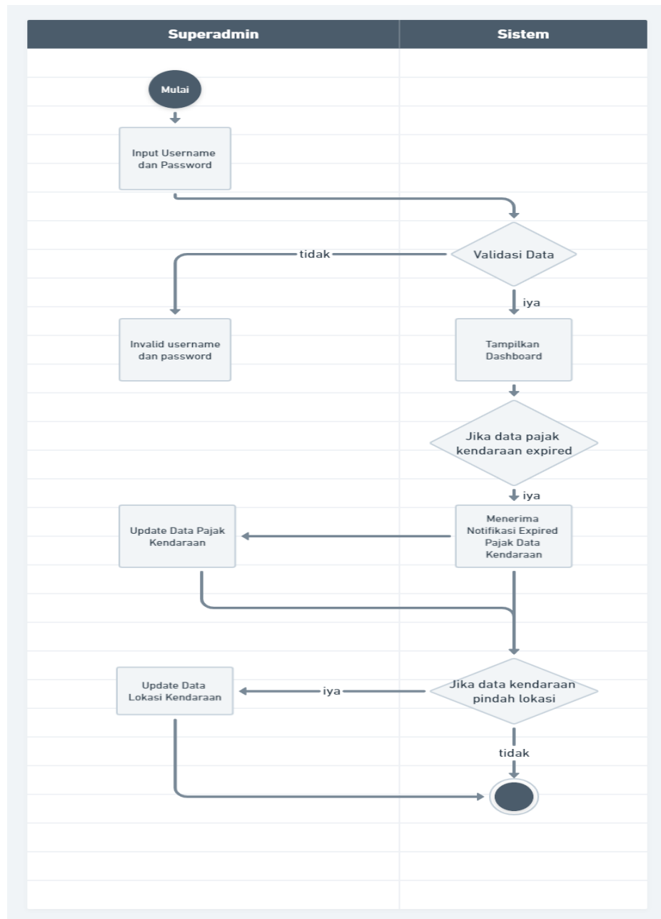
Gambar 4.3 Activity Diagram SuperAdmin Login
