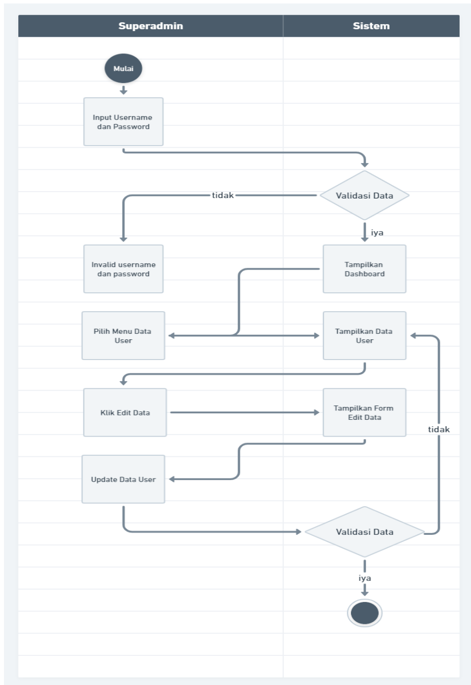
Gambar 4.5 Activity Diagram SuperAdmin Edit Akun User
