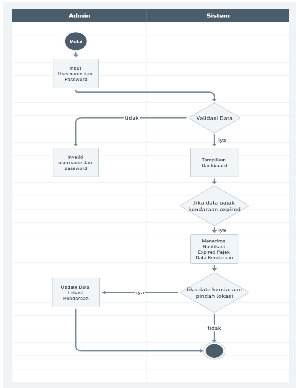
Gambar 4.2 Activity Diagram Admin Login
