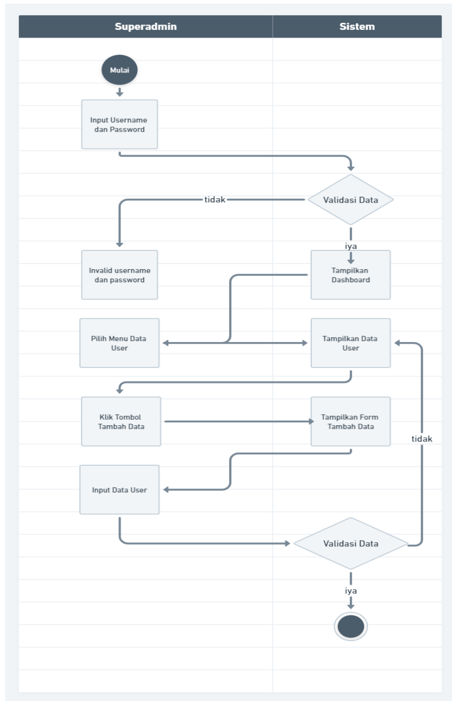
Gambar 4.4 Activity Diagram SuperAdmin Create Akun User
