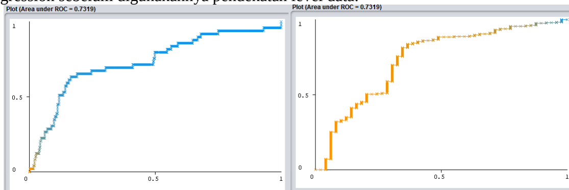
Gambar 1. ROC Class False & Class True Algoritma Logistic Regression
