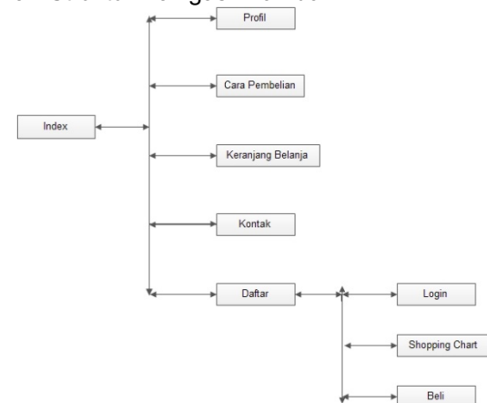
Gambar 5. Struktur Navigasi Member
