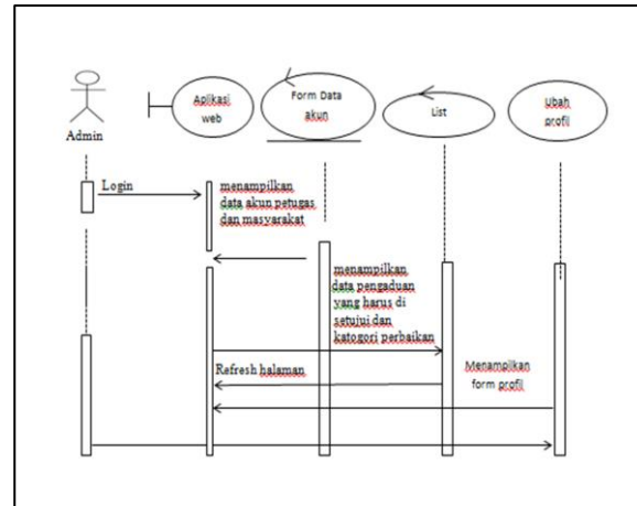
Gambar 9. Rancangan Sequence Diagram Admin
