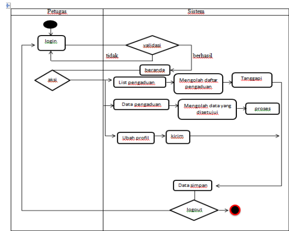
Sumber : Hasil Penelitian (2021) Gambar 4. Activity Diagram Petugas
