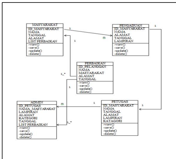
Gambar 8. Rancangan Class Diagram
