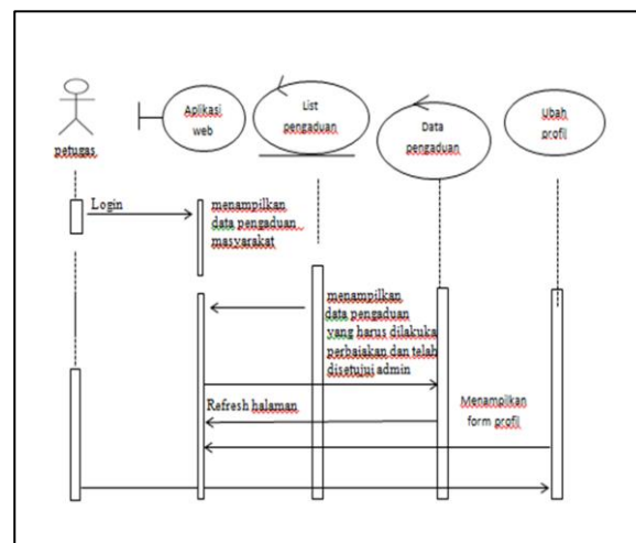
Gambar 10. Rancangan Sequence Diagram Petugas
