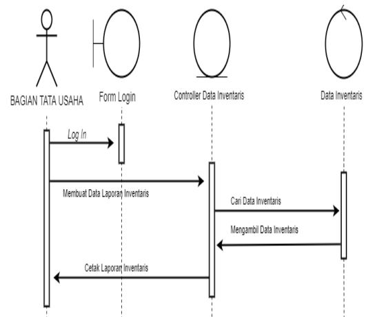
Gambar 12. Sequence Diagram Proses Laporan
