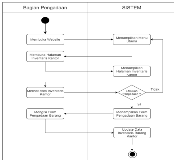
Gambar 5. Activity Diagram Pengadaan Barang
