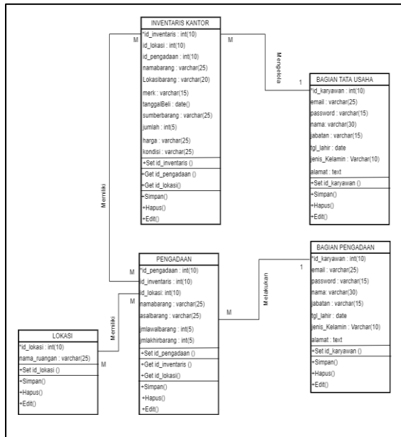
Gambar 9. Class Diagram
