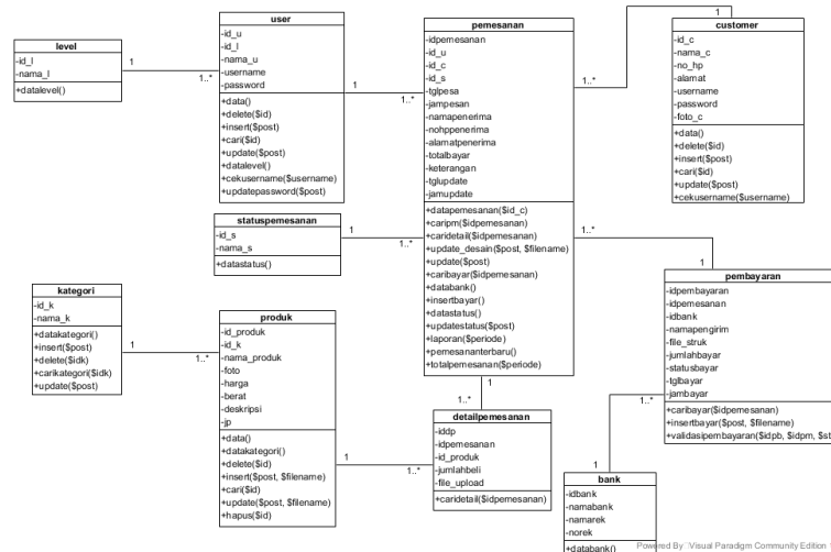
Gambar 12. Class Diagram
