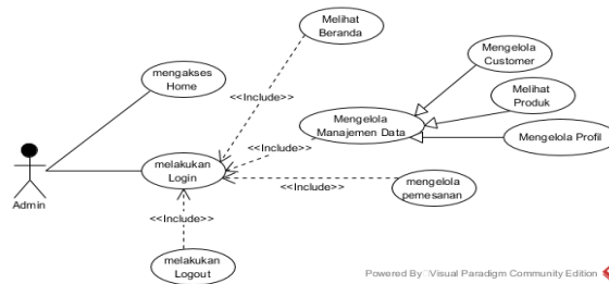
Gambar 2. Use Case Diagram Admin
