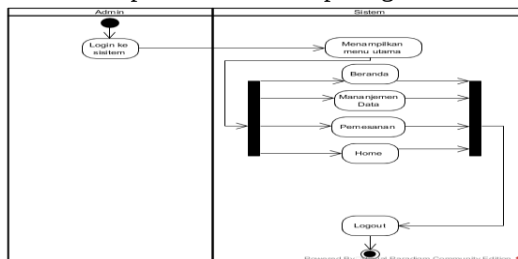
Gambar 6. Activity Diagram Menu Admin
