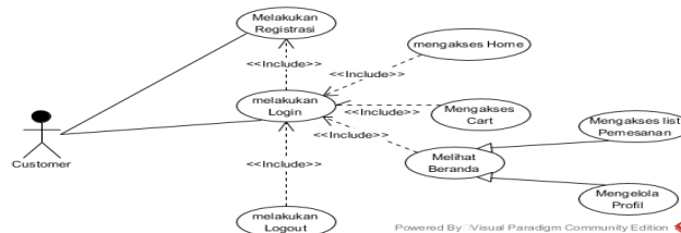
Gambar 3. Use Case Diagram Costumer
