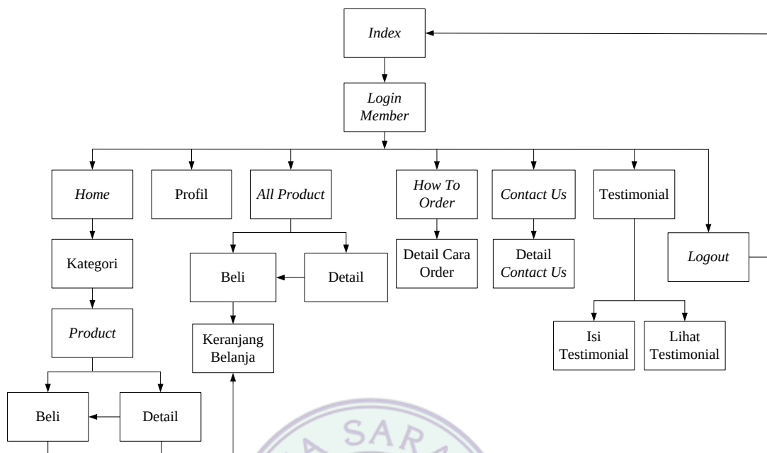
Gambar III.50. Struktur Navigasi Member
