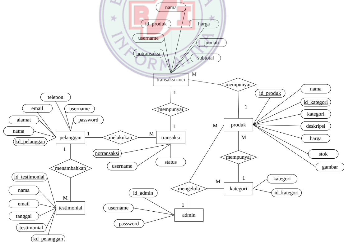
Gambar III. 47. Entity Relationship Diagram (ERD)
