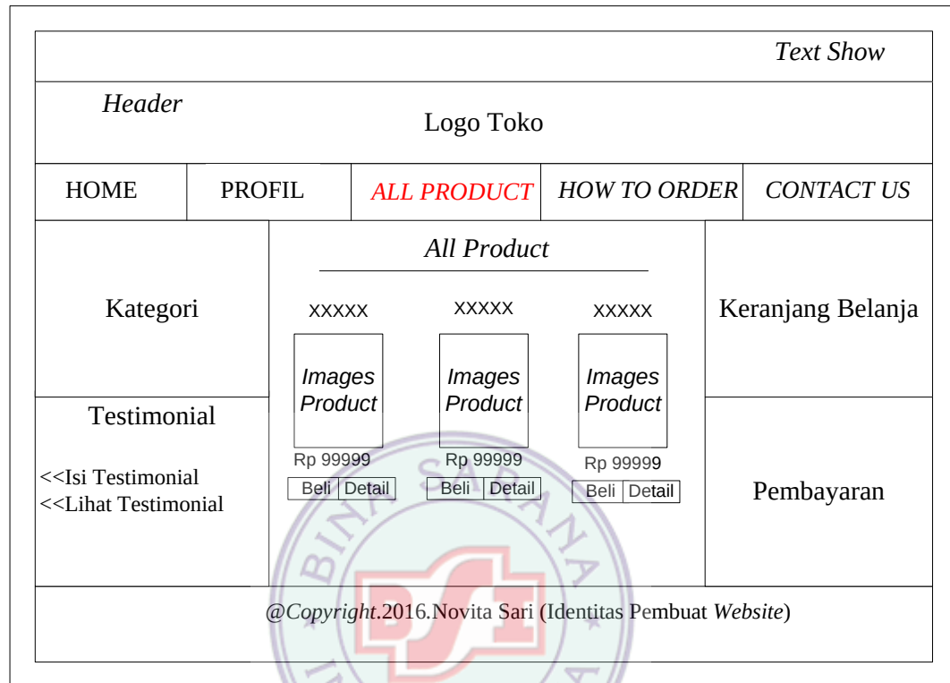
Gambar III.21. Rancangan Antar Muka All Product
