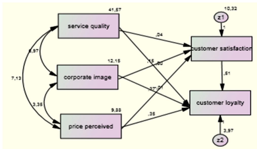
Figure 1. Initial Path Diagram Model
