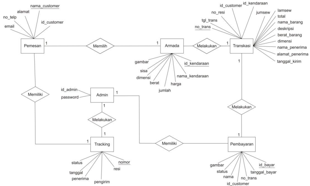
Gambar III.8. ERD (Entity Relationship Diagram)
