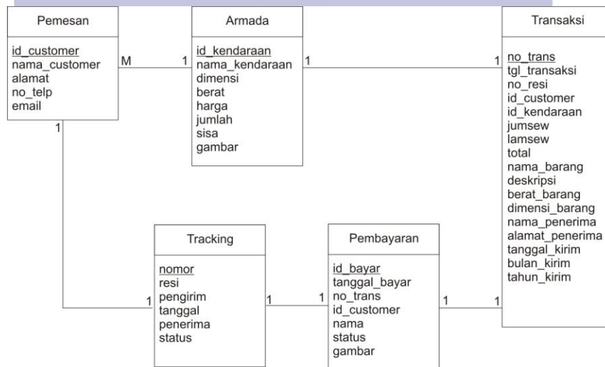
Gambar III.9. LRS (Logical Record Strukture)
