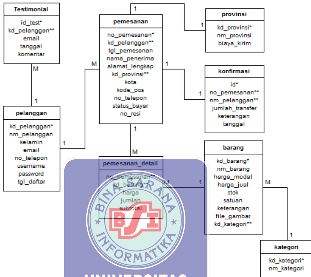
Gambar III.54. LRS (Logical Record Structure)
