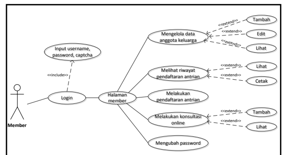
Gambar 2. Use Case Diagram Mengelola Halaman Member
