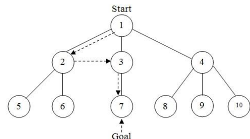
Gbr 6. Best-first-search
