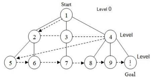
Gbr 5. Breadth-first-search
