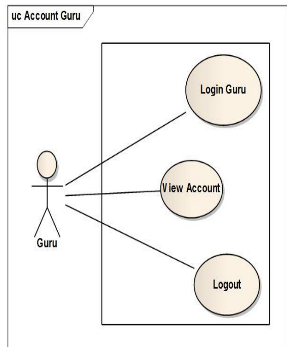
Gambar 8. Use Case Diagram Guru
