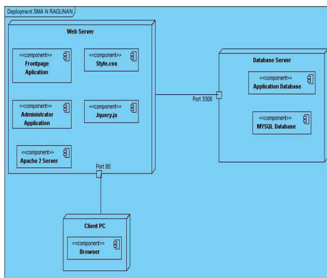
Gambar 7 Deployment Diagram
