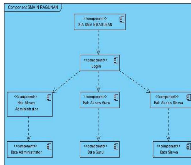
Gambar 6 Component Diagram
