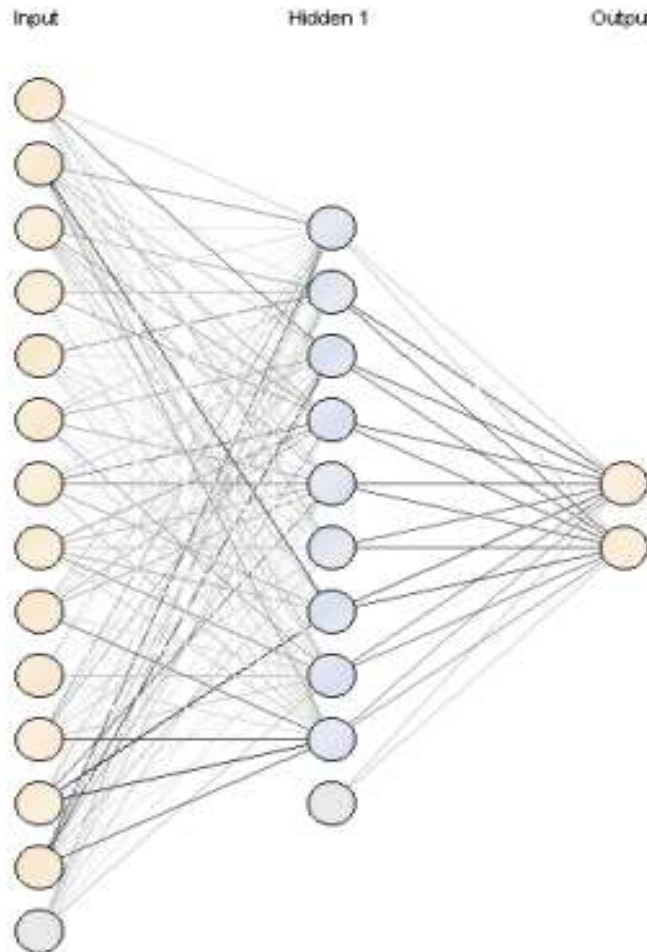
Gambar 5. Neural Network
